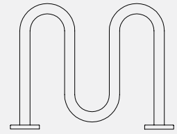
BIKE RACK 125 2-7/8" O.D. Tubing
